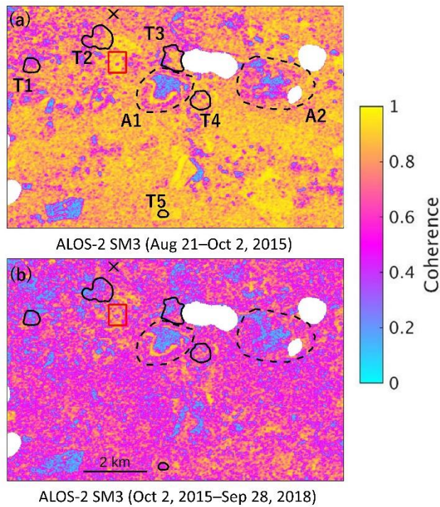
Fig. S2 A comparison of coherence at different temporal baselines derived from ALOS-2 SM3 data spanning (a) 42 days and (b) 3 years.
