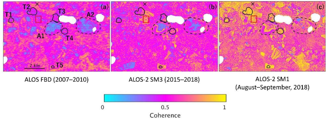
Fig. S1 Averaged coherence map derived from (a) ALOS FBD, (b) ALOS-2 SM3, and (c) ALOS-2 SM1 data.
