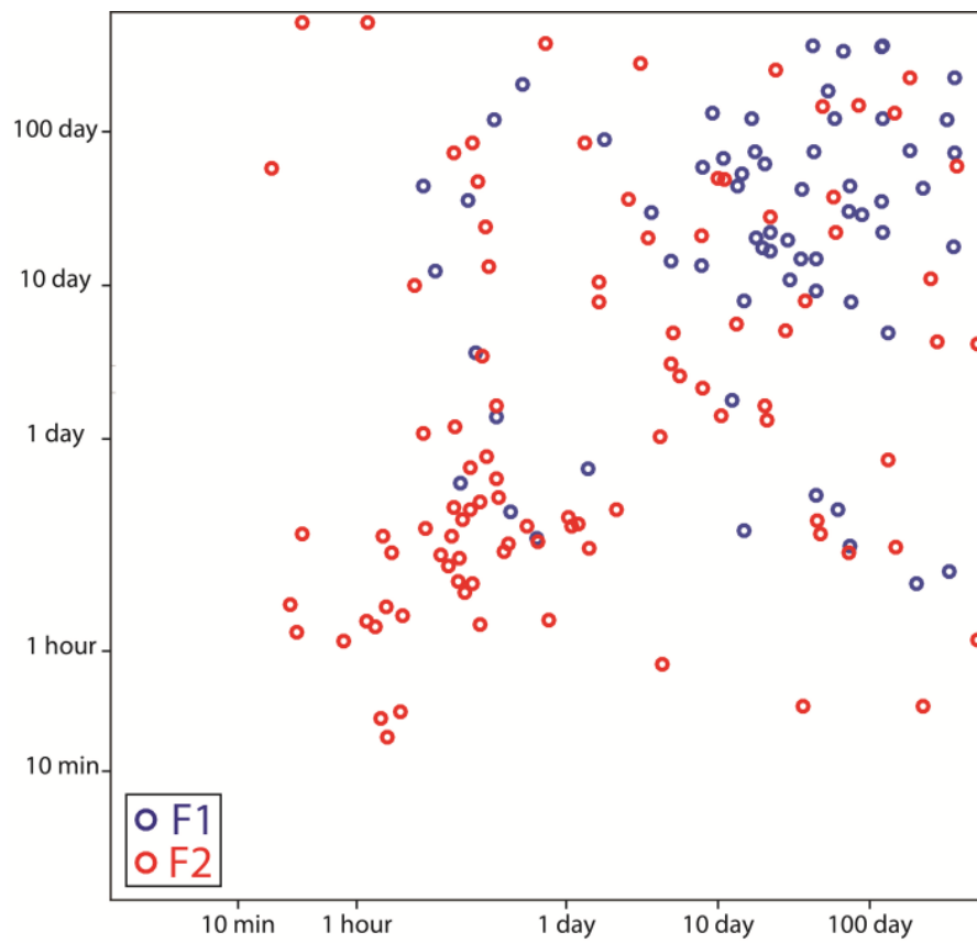
Additional file 5. Time map of two VLP families (F1 and F2). Axes indicate the time intervals between each VLP and its preceding (x axis) and subsequent (y axis) events. Swarm and intermittent VLPs are separately clustered.
