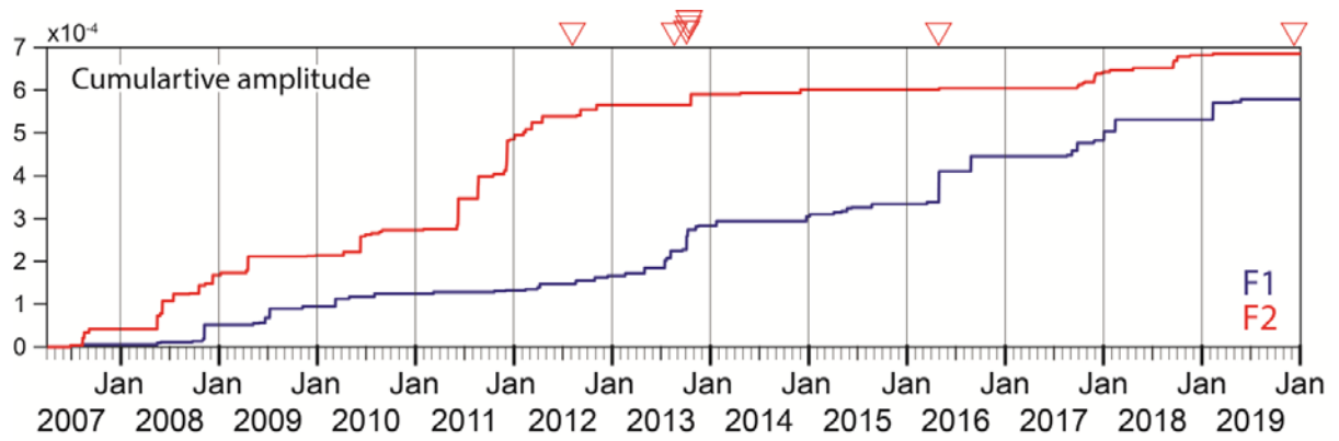
Additional file 5. Cumulative amplitude of F1 (blue) and F2 (red). The seven eruptions are denoted by reversed triangles (red).
