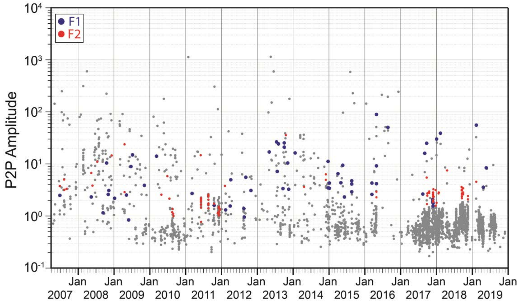
Additional file 3. Template matching results (gray dots) without semblance and SNR filtering. This catalogue includes two families (F1 and F2) as well as teleseismic data and lower SNR events. The vertical axis is peak-to-peak (P2P) amplitude ( \mu\text{m/s} ) computed using the vertical component of WIZ station.
