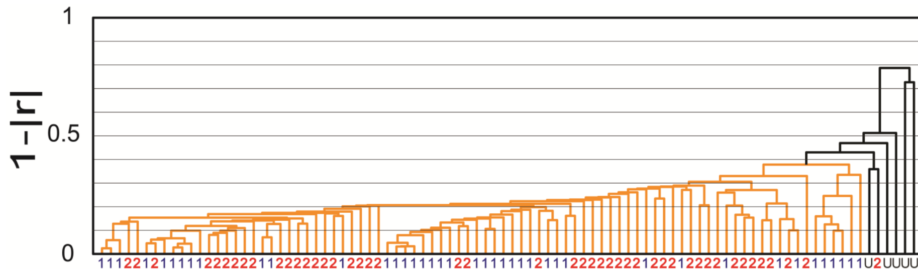
Additional file 2. A dendrogram based on the absolute value of correlation coefficient. Two families (F1 and F2) belong to a cluster (orange lines) except for one low SNR waveform, and all U events denote black lines.
