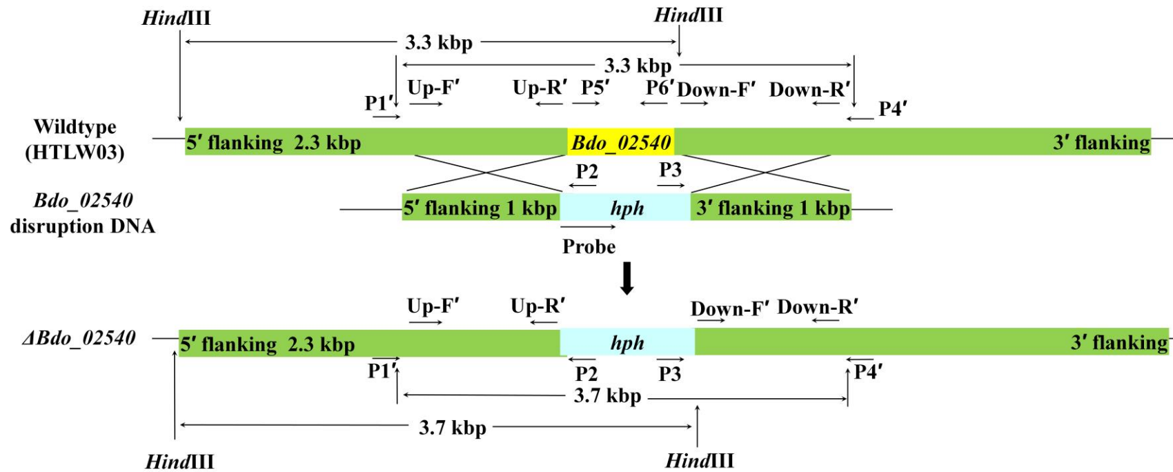
Fig. S3 Genomic details regarding Bdo_02540
