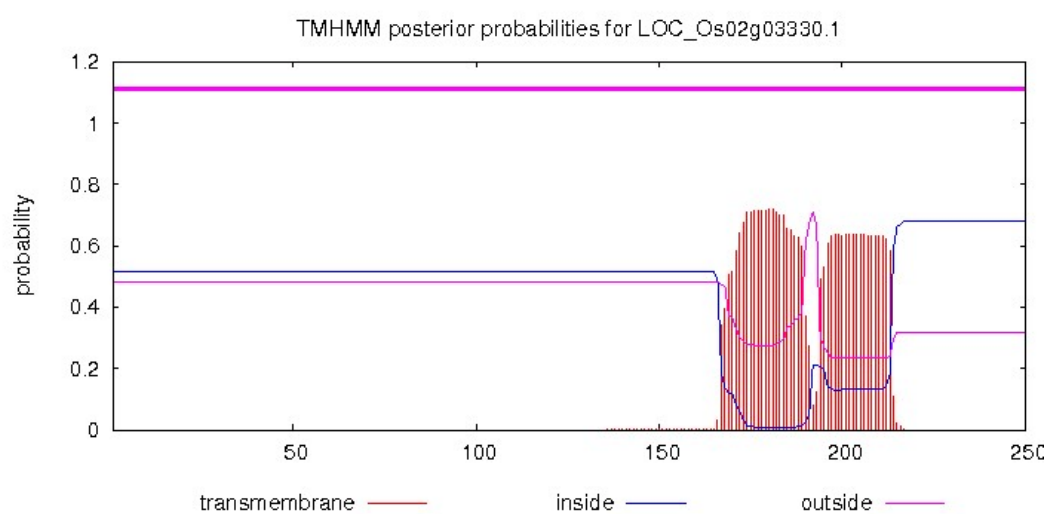
Additional file 9: Figure S5. Predicted transmembrane domain of the OsLIL3 (LOC_Os02g03330) protein.
